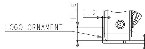
DETAIL B SCALE 1/2
